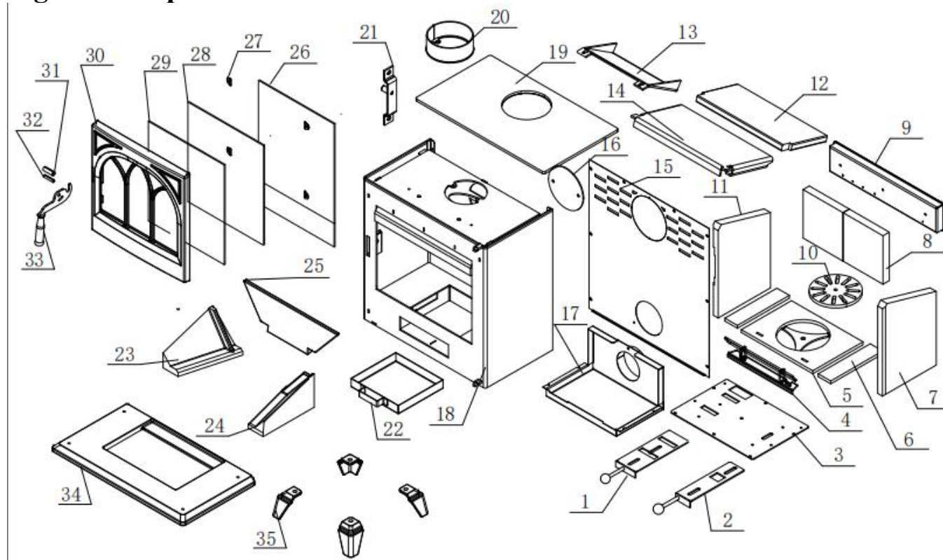
Figure 2 -Exploded view
